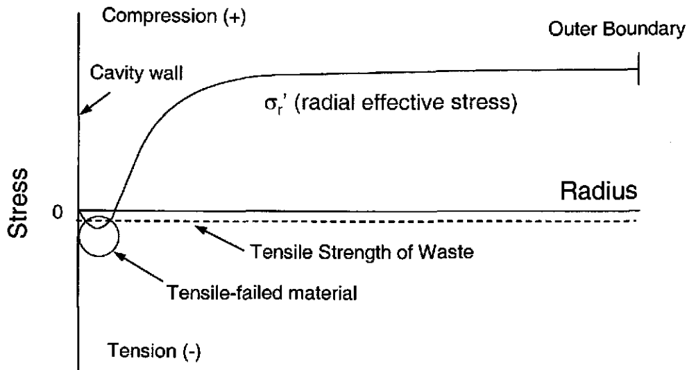
Figure 2-6. Drawing of a theoretical radial effective stress curve. Material is subject to tensile failure where \sigma_r'(r) < T_s .
